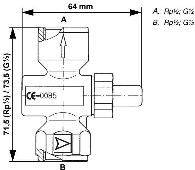
Figure 1: Dimensions et raccords (Rp 1/2; G 1/2)
