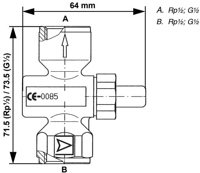
Fig. 1: Dimensions and connections ( Rp\frac{1}{2}; G\frac{1}{2} )
